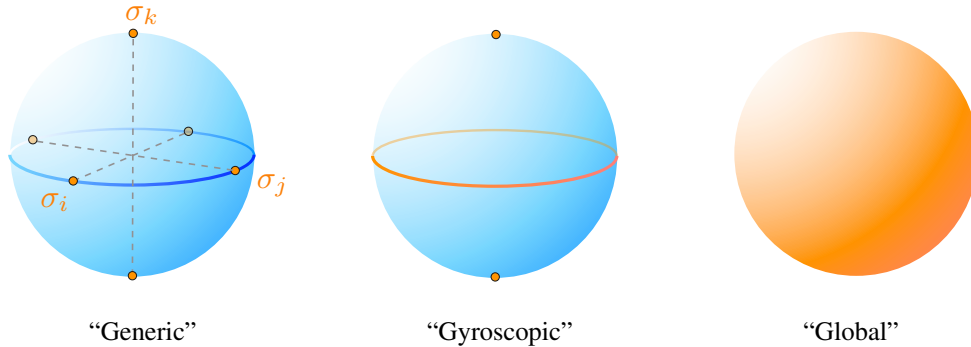
Figure 9: Admissible configurations
