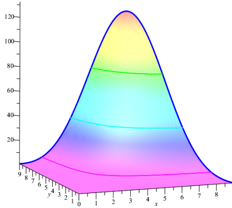
Figure 3: Pascal's Surface
