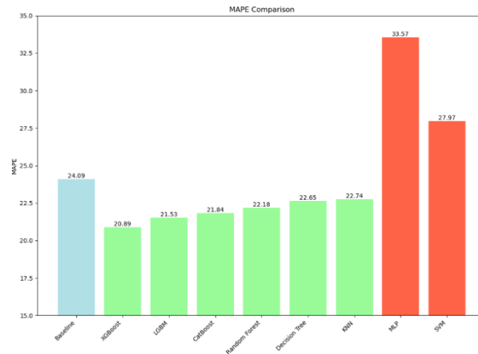
Figure 1. MAPE Comparison Graph of the Baseline and Machine Learning Models
